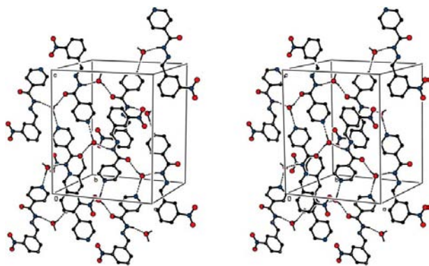
Figure 4 A stereoview of part of the crystal structure of compound (I), showing the formation of a hydrogen-bonded sheet parallel to (010). For the sake of clarity, H atoms bonded to C atoms have been omitted.
